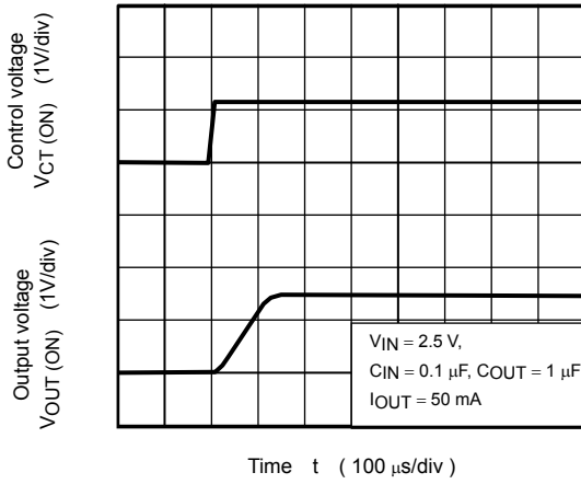
TCR5SB15A (Turn on wave form)
